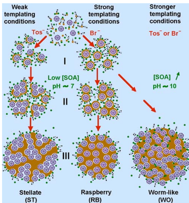
Scheme 1. Synthesis Mechanisms at Low or High SOA Concentration (pH \approx 7 or 10) and Tos - (left) or Br - (middle) (template counterion is not represented here) a
